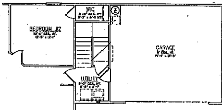
FIRST FLOOR LAYOUT W/ OPT. BONUS RM.
